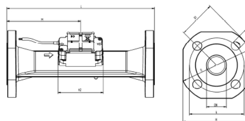
Dimensions qp 15.0
