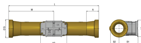
Dimensions qp 3.5- 10.0
