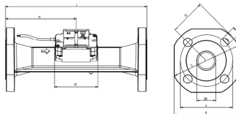
Dimensions qp 15.0
