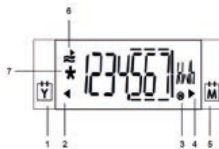
Fig. 6: LCD-display
