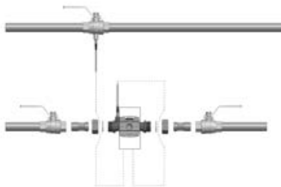
Fig. 2: Example for installation with ball valve and meter with 110 mm armature
