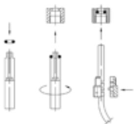
Fig. 5: Montering adaptersett
